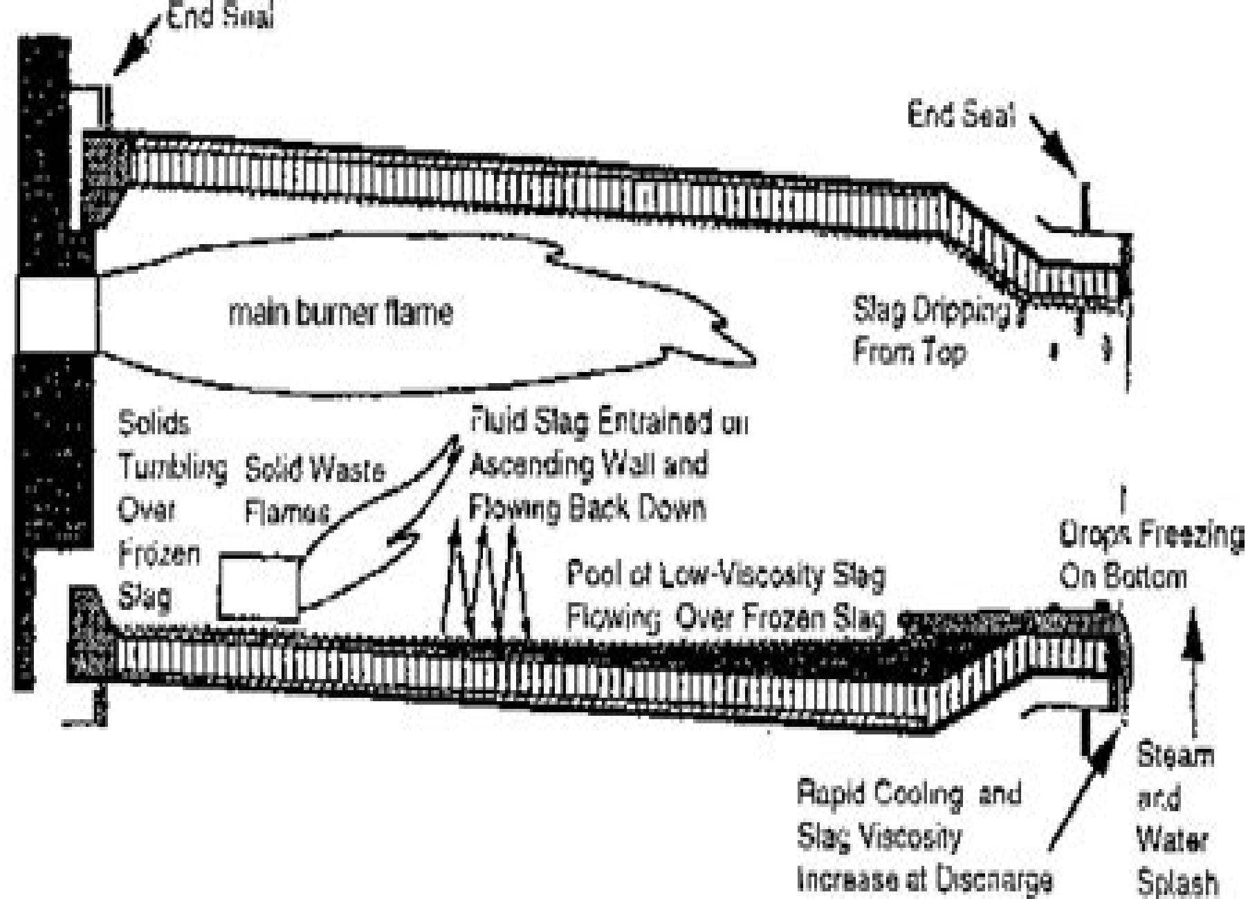
Figure 2: Illustration of the rotary kiln (Veranth et al 1996)
