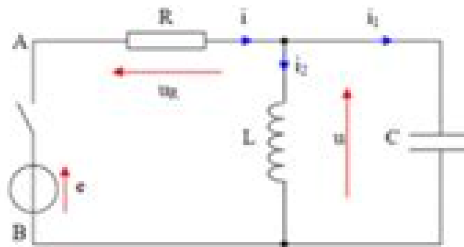
Figure 1: Parallel RLC circuit
