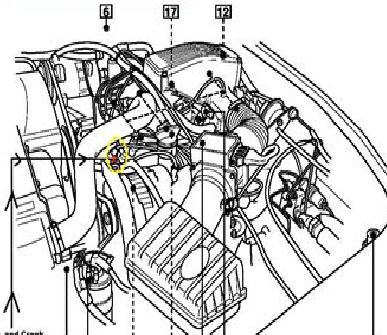
Location of Dist and Crank shaft ( crank ) sensor
