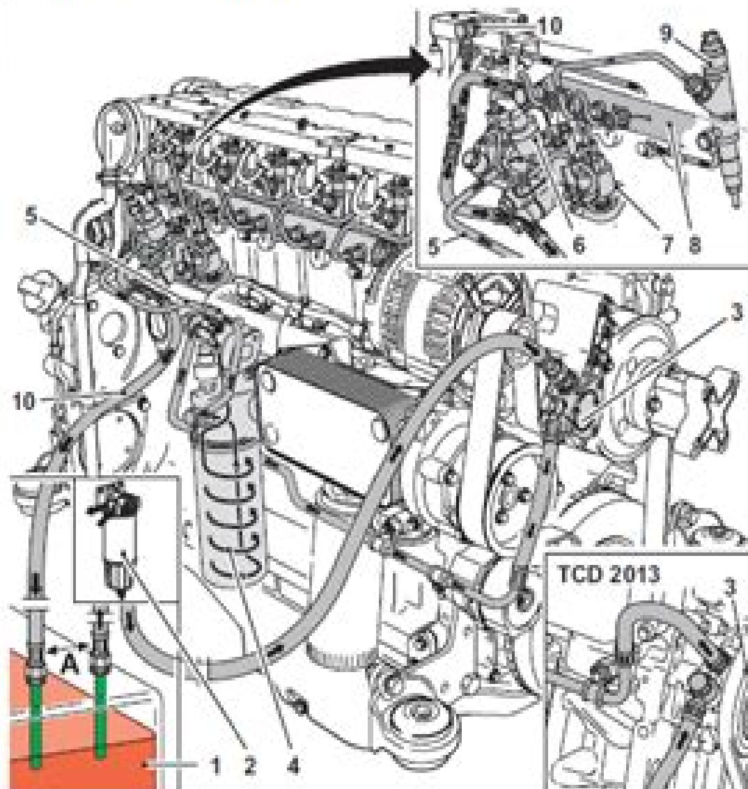
Fuel schematic (example)
