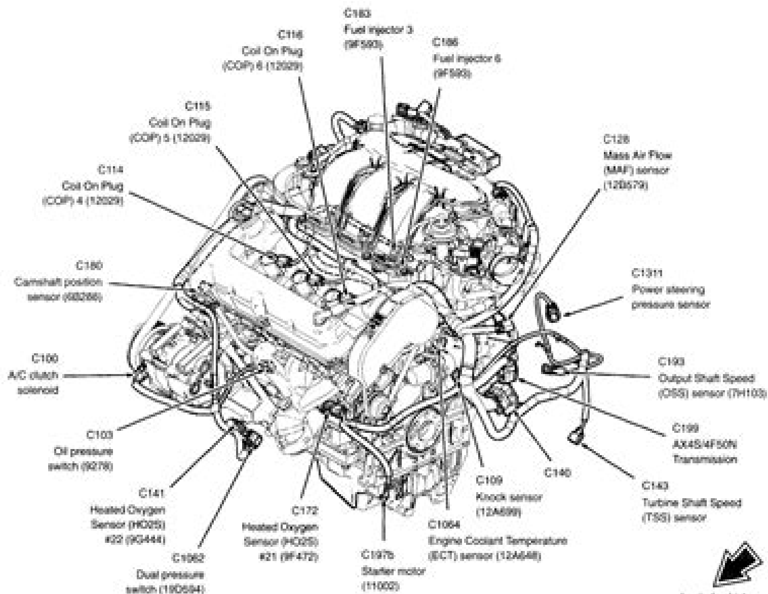
4V engine, front
