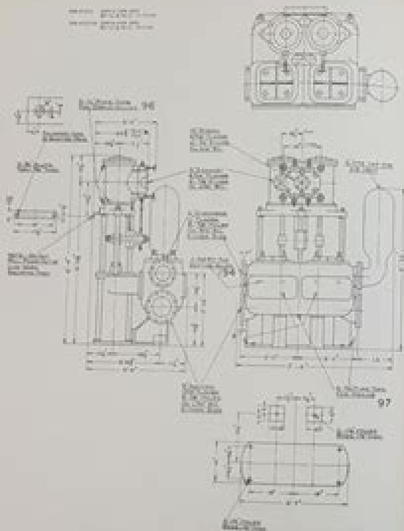
10-11-12 Fuel Oil Transfer Pump Head
