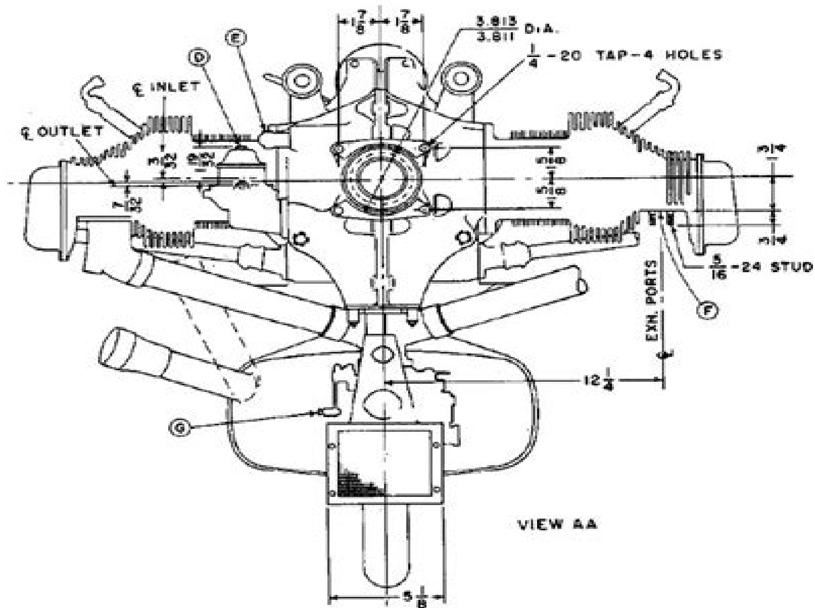
Figure 13. Installation Drawing for -12, -14 & -16 Models, Front View.
