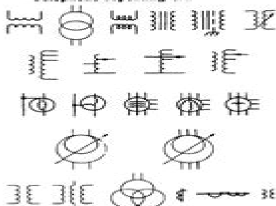
6.4 Transformer Telephone induction coil Telephone repeating coil
