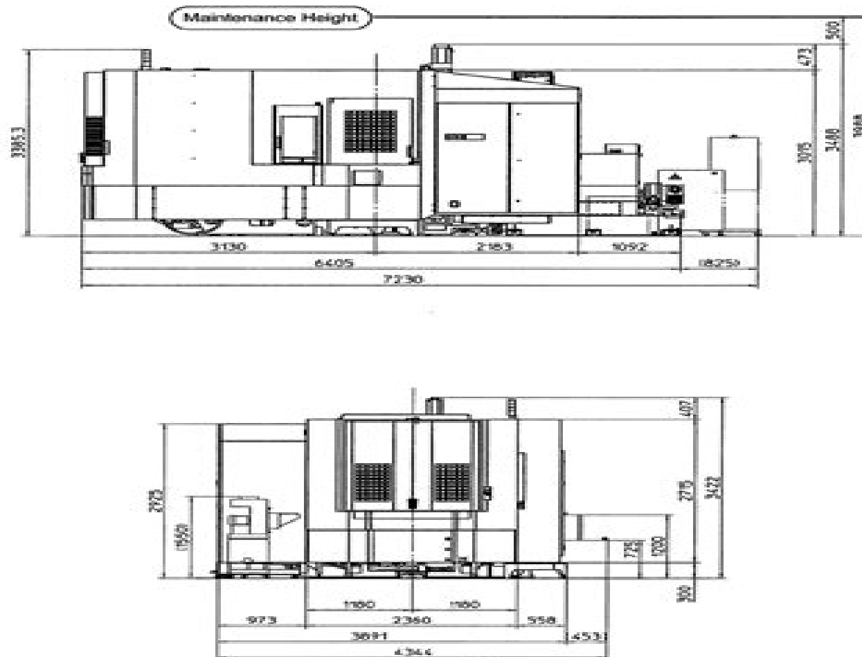
a82 General View: Tool Magazine A60, Left-Discharge Conveyor
