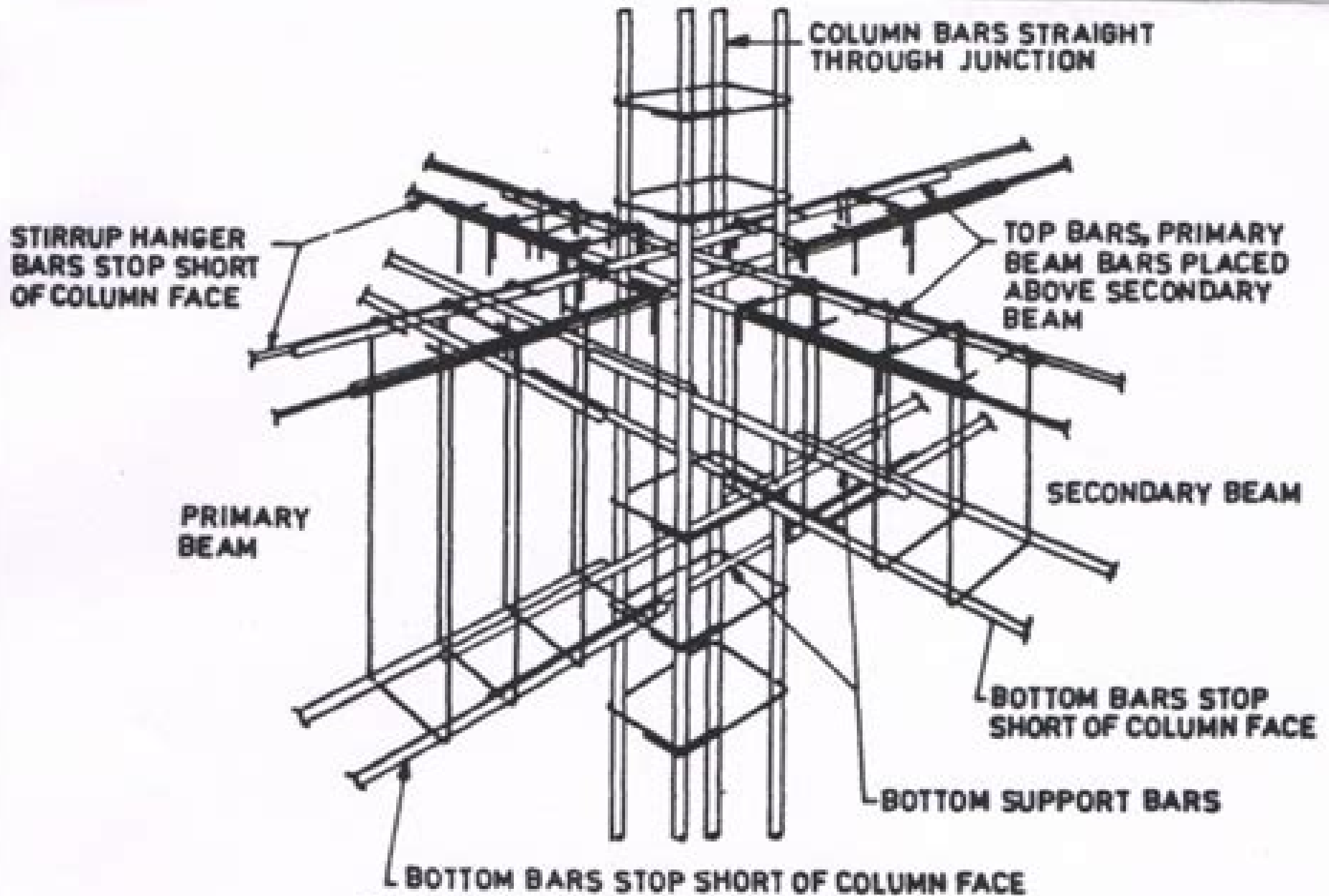
FIG. 7.13 BEAM-COLUMN INTERSECTION
