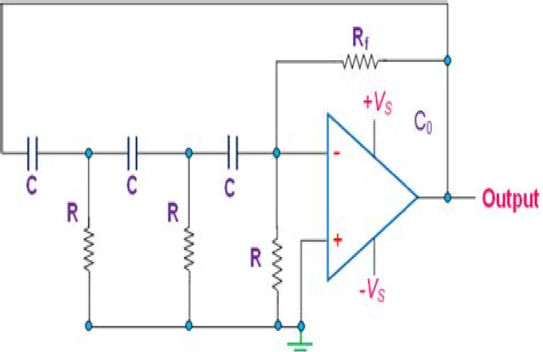
Figure 3 RC Phase-Shift Oscillator Using an Op-Amp
