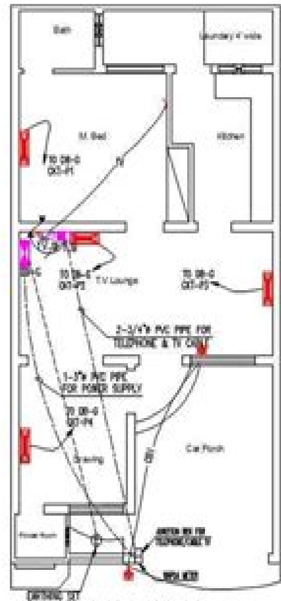
POWER TELEPHONE TV & A/C WIRING SYSTEM LAYOUT FOR GROUND FLOOR PLAN
