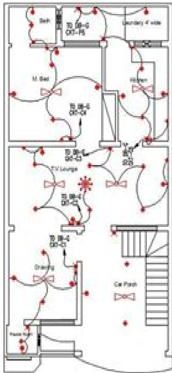
LIGHTING PLAN Ground Floor
