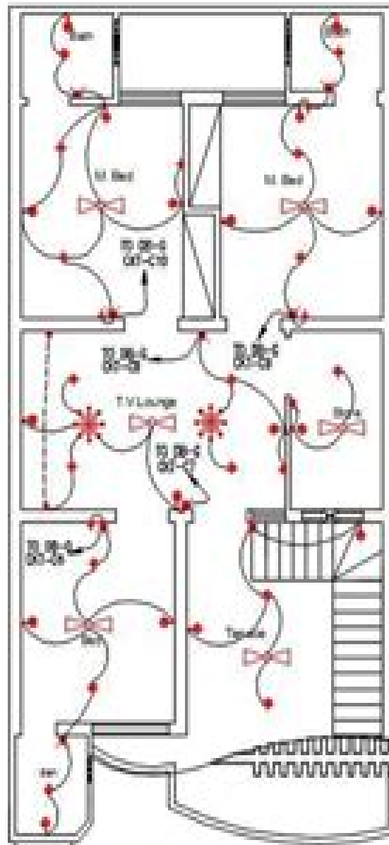
LIGHTING PLAN First Floor
