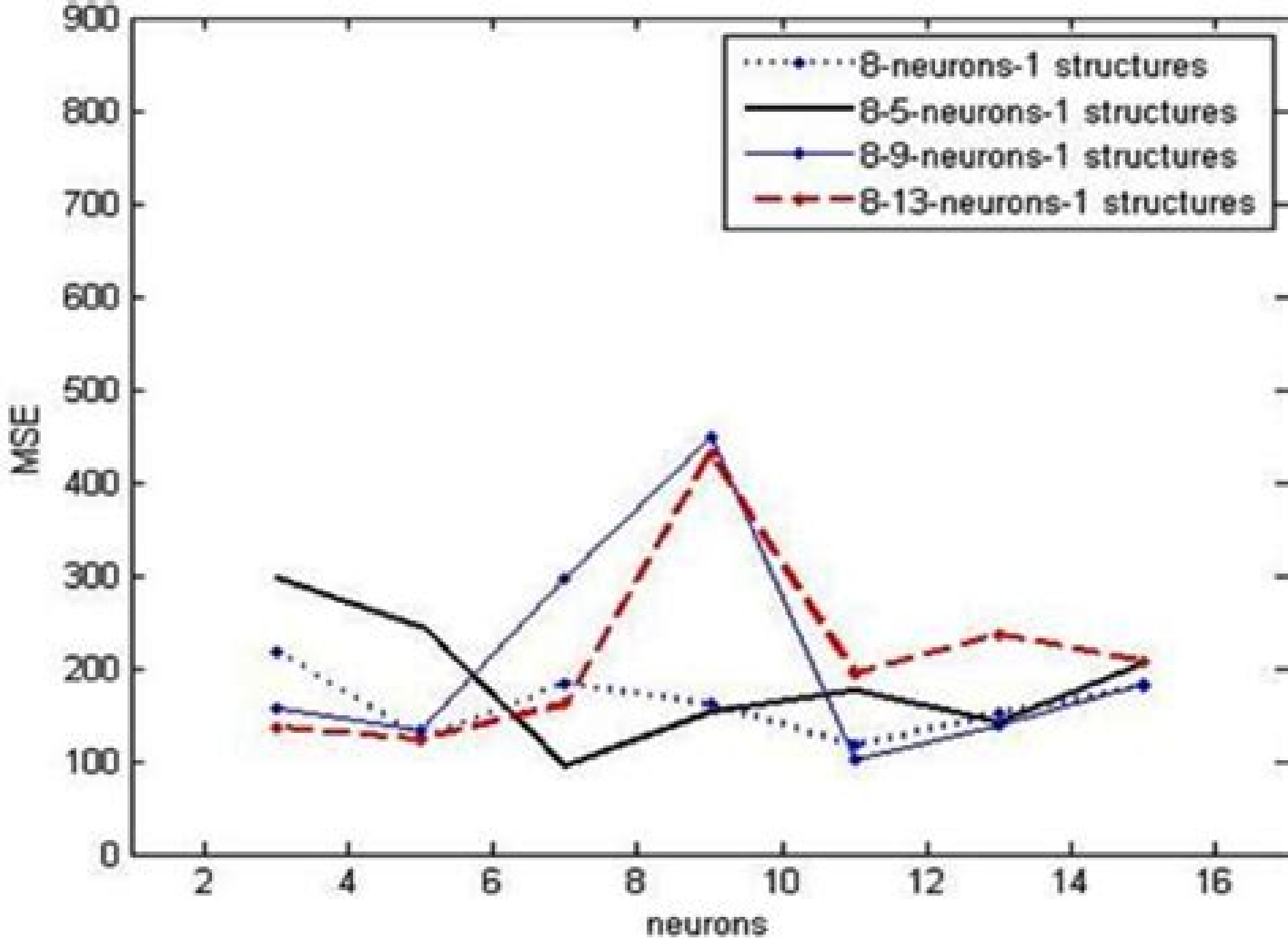
Figure 1: Comparison of the performance of different neural network structures.
