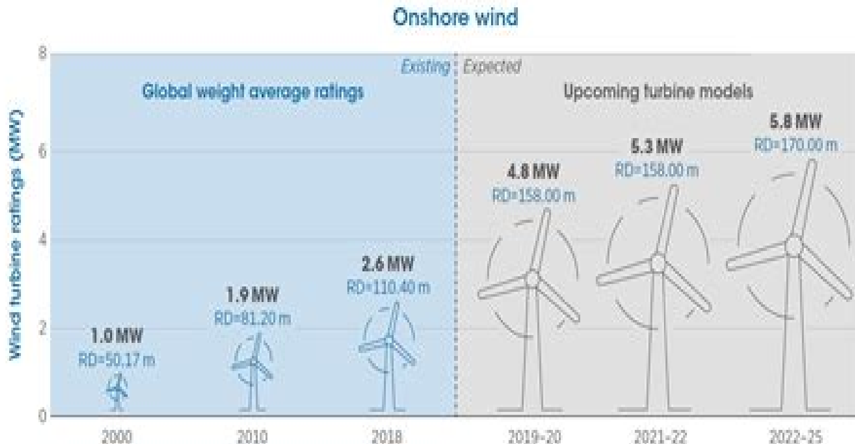
Figure 18: Ongoing innovations and technology enhancements towards larger-capacity turbines, increased hub heights and rotor diameters would improve energy yields and reduce capital and operation costs per unit of installed capacity.
