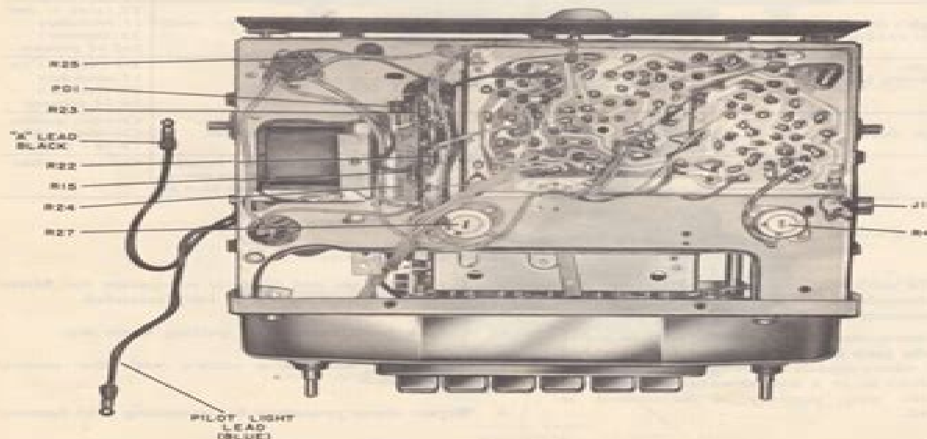
Figure 2. Bottom View, Showing Location of Parts
