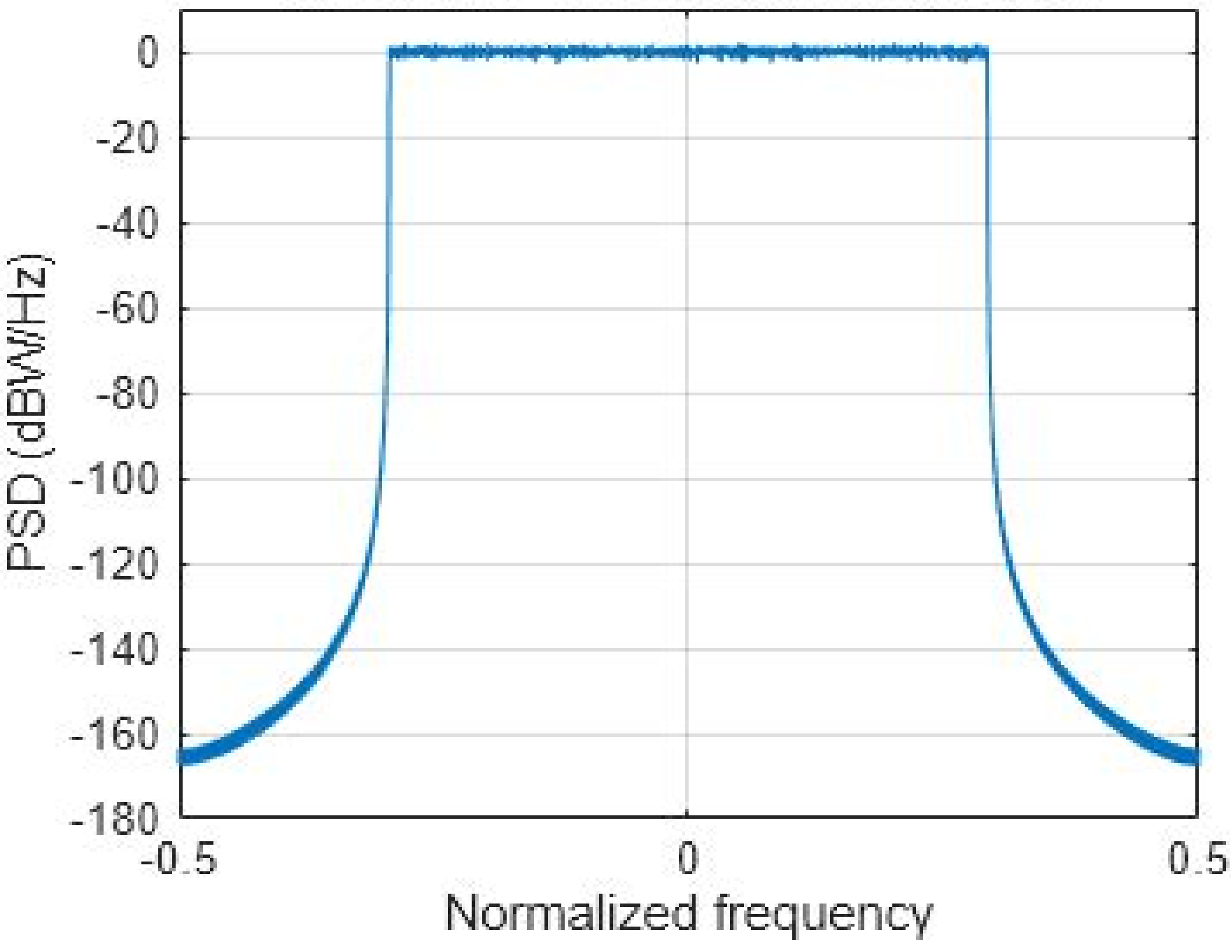
FBMC, K = 4 overlapped symbols
