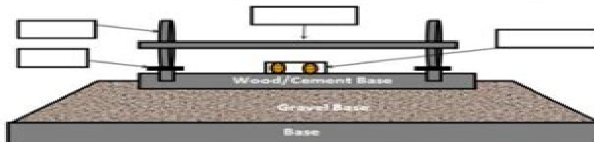
Fig 3. Cross section of wheels on tracks and pipe encompassing Fiber Cables located between tracks
