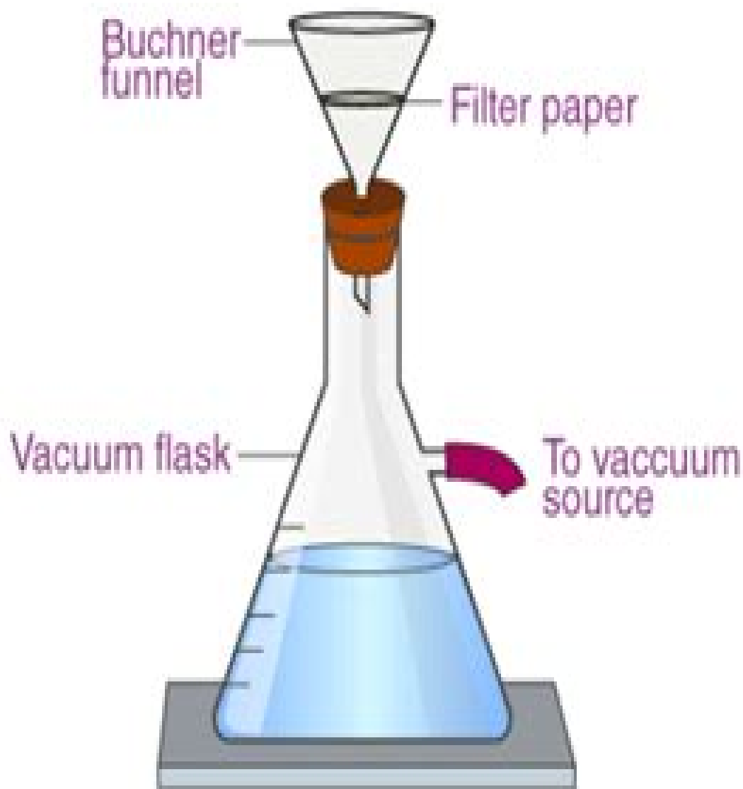
Gravimetric Analysis Apparatus
