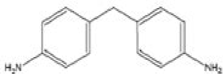
4,4'-methylenedianiline
