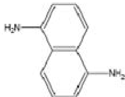
1,5-diaminonaphthalene
