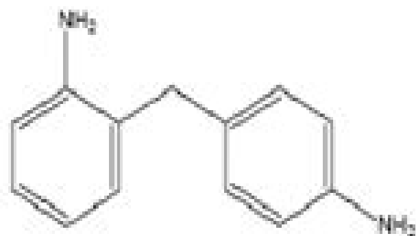
2,4-methylenedianiline
