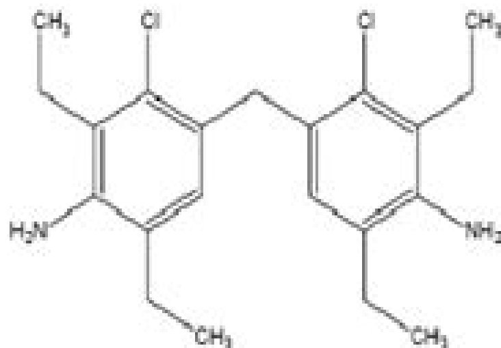
4,4'-methylenebis(3-chloro-2,6-diethylaniline)
