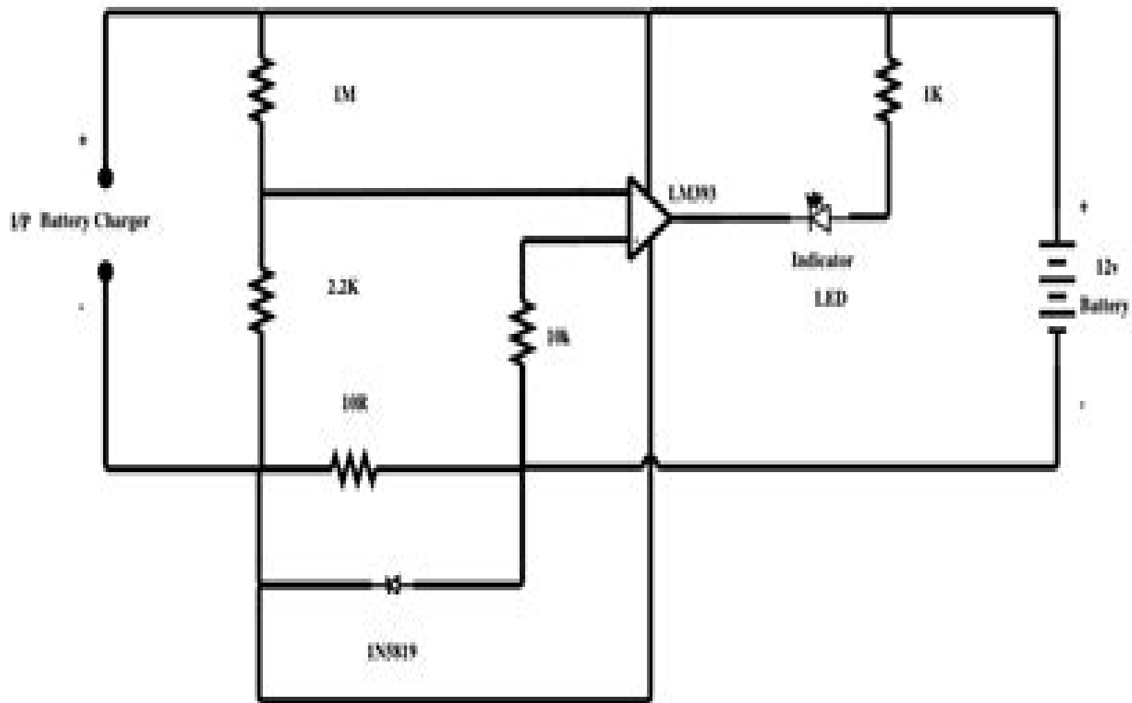
Battery Charging Indicator Circuit
