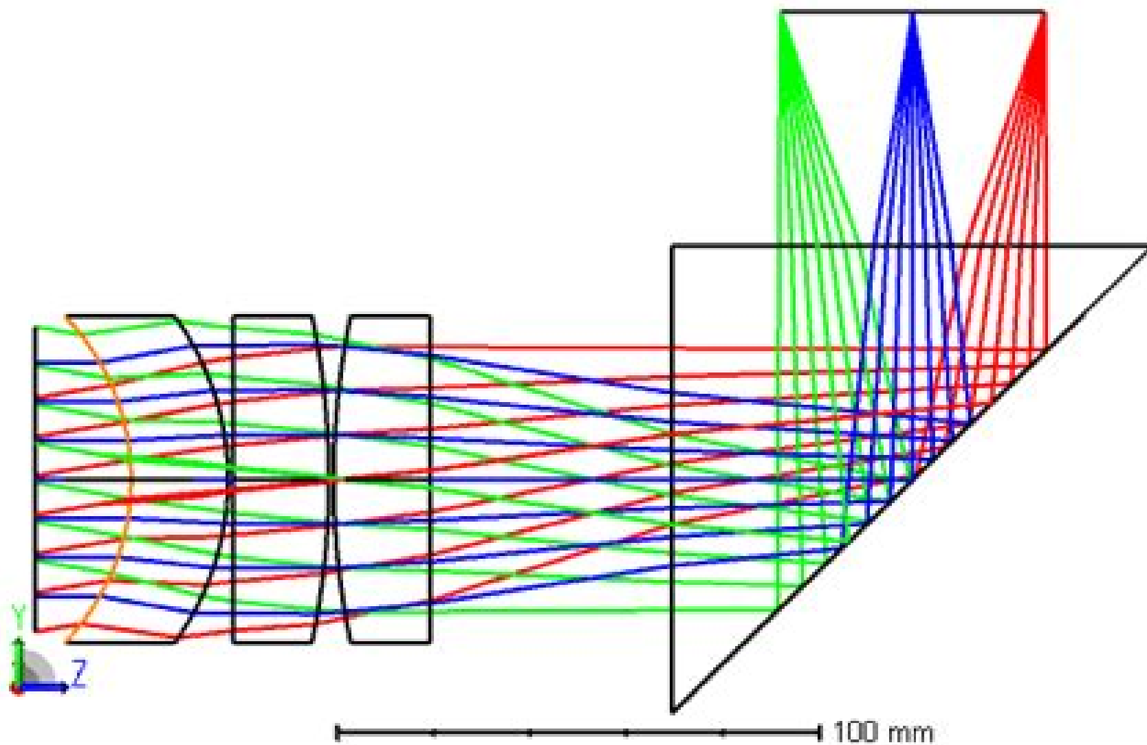
3D Layout
