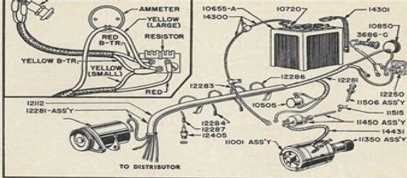
Fig. 11 — Wiring Diagram
