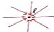
Negative divergence
