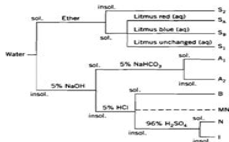
Figure 1. Classification of organic compounds by solubility (see Table 1 for compounds comprising each class). sol. = soluble; insol. = insoluble; litmus red is at pH below 4.5 and blue above 8.3.
