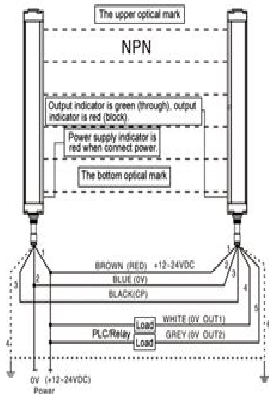
NPN double outputs, four & six wires connection
