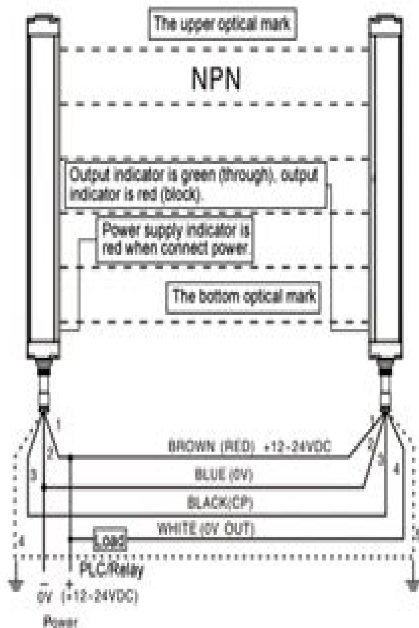
NPN single output, four & five wires connection
