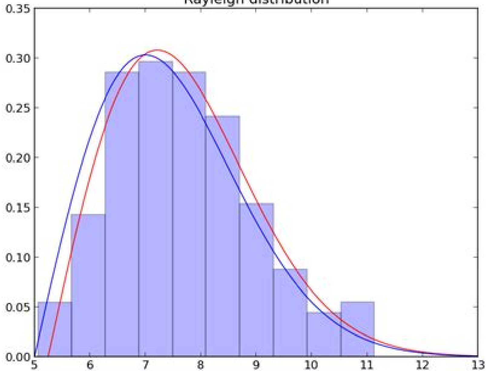
Rayleigh distribution
