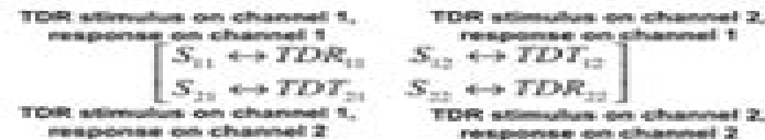
Figure 1. Relationship between the TDR/T data and the single-ended S-parameters
