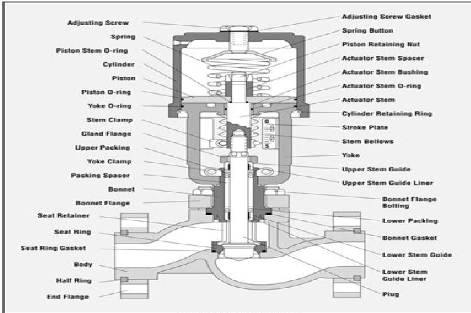
Figure 2: Mark One Control Valve
