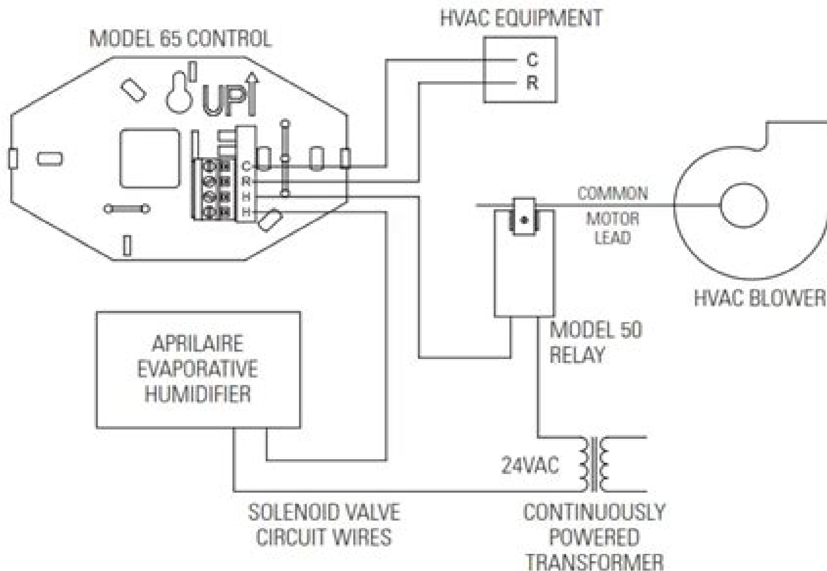
FIGURE 5 – Alternate Wiring for Model 65 Control and Evaporative Humidifier
