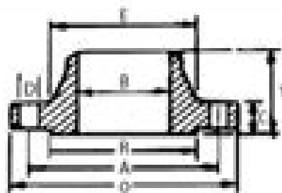
Welding Neck
