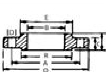
Slip-On
