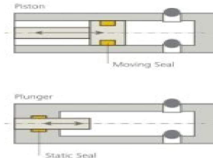
Figure 3.3: API 674, Piston and plunger pumps
