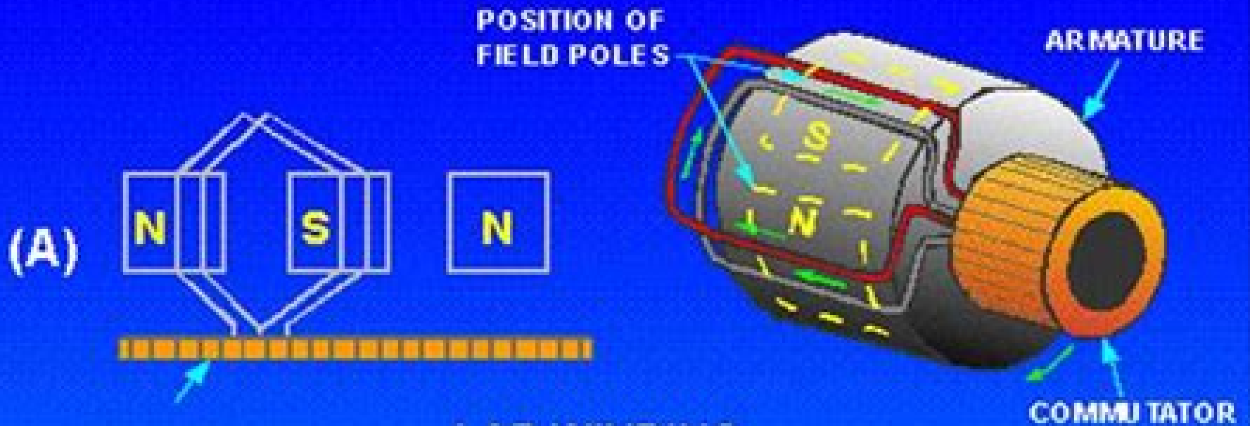
LAP WINDING
