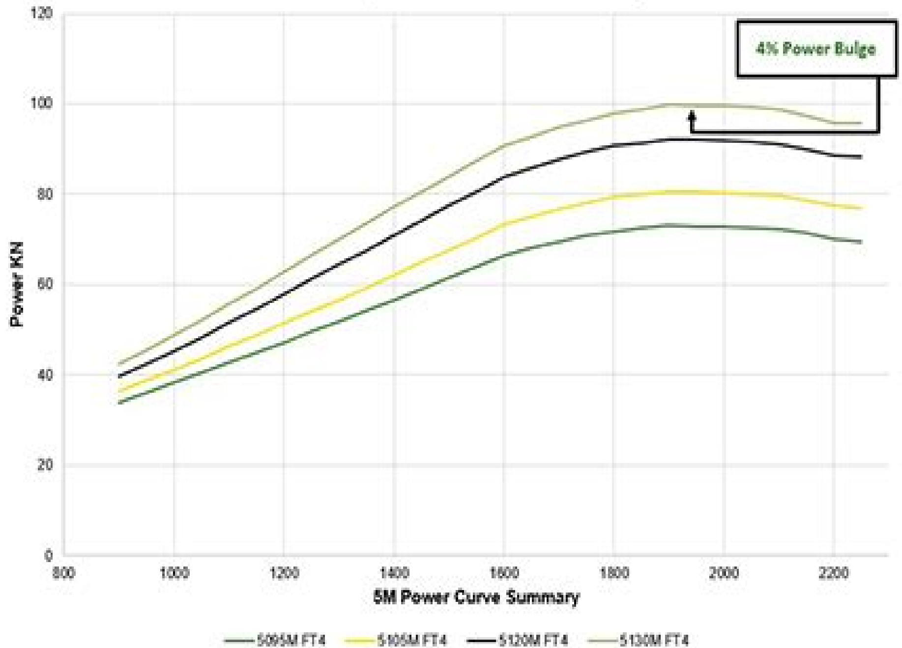
5M FT4 Engine Power Curve Summary
