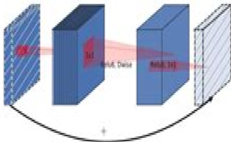
Mobilenet V2: bottleneck with residual
