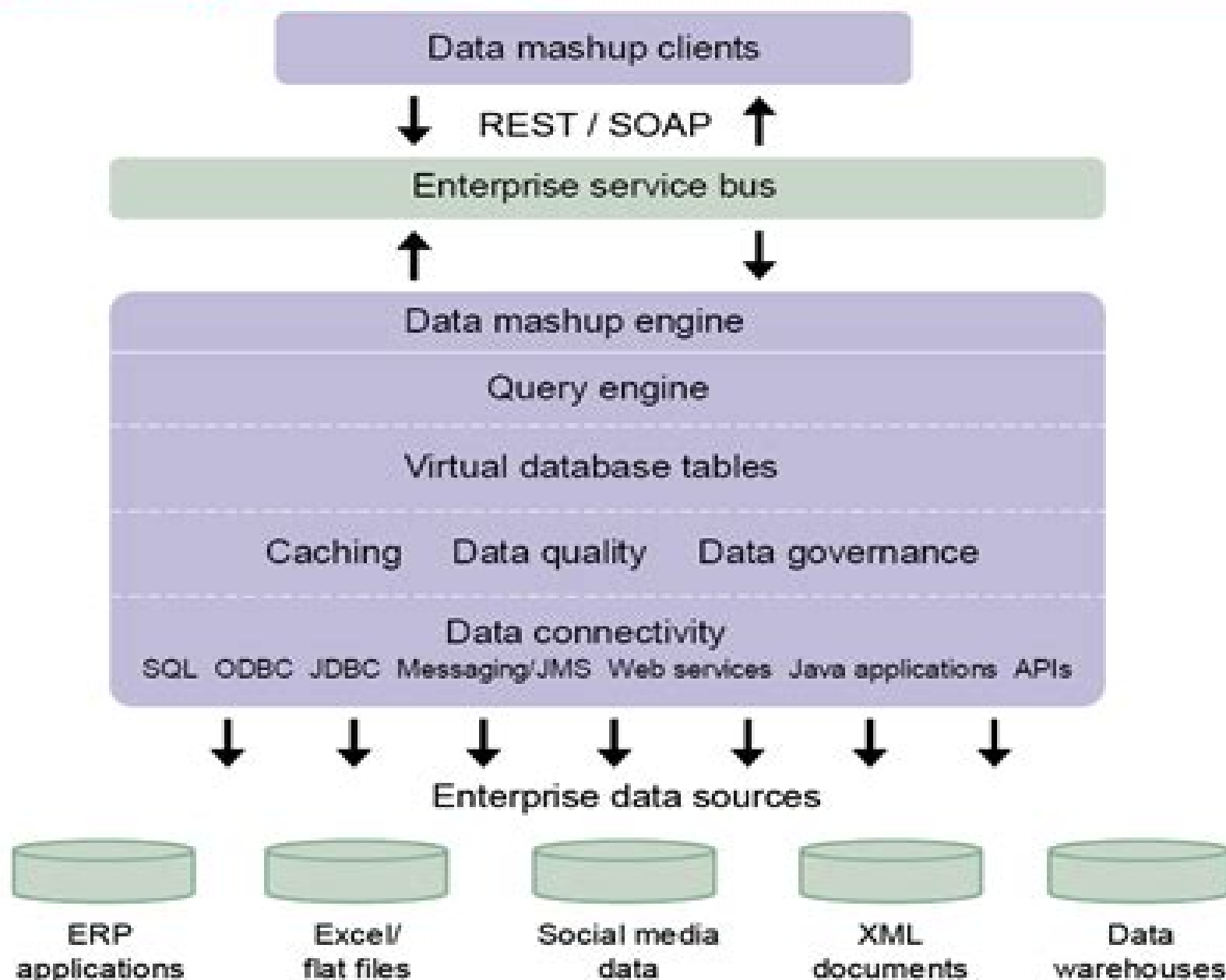
Figure 1: Anatomy of a data mashup
