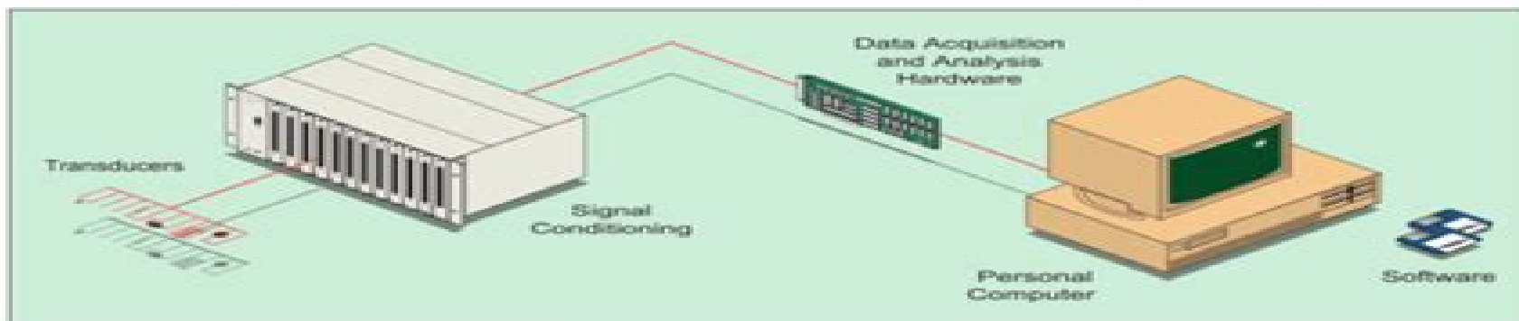
Figure 1. The Typical D/AQ System
