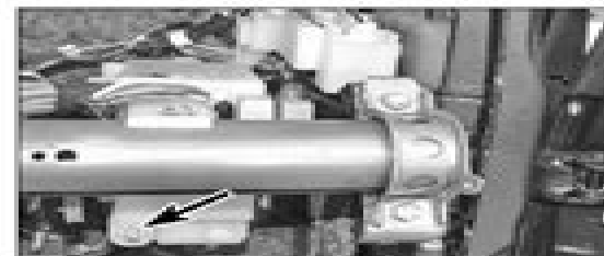
26.25 Undo the wiring block lower mounting bolt (pictured with facia removed)
