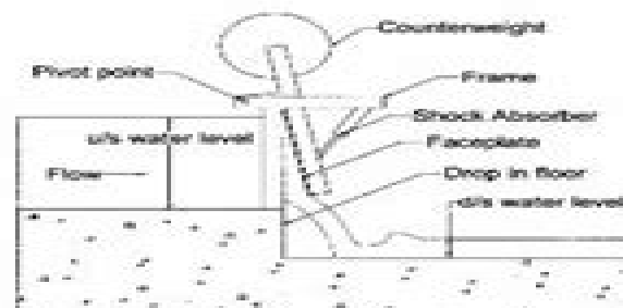
FIG. 1. Side View of Flap Gate
