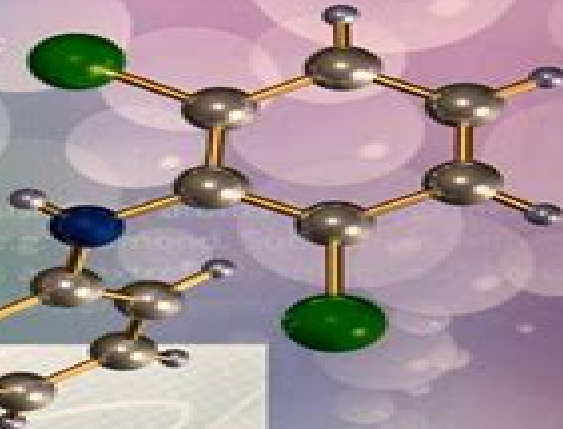
Polyatomic molecule
