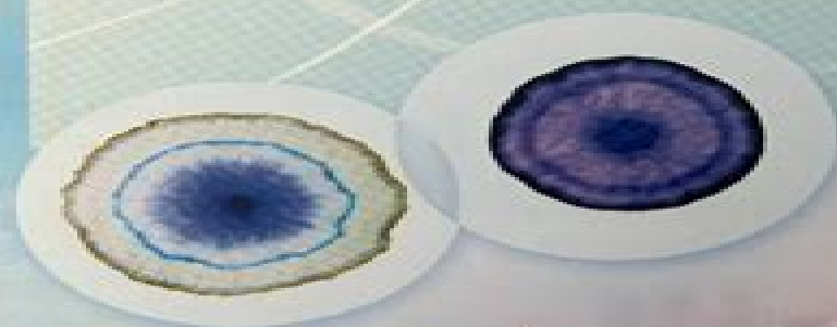
Chromatography
