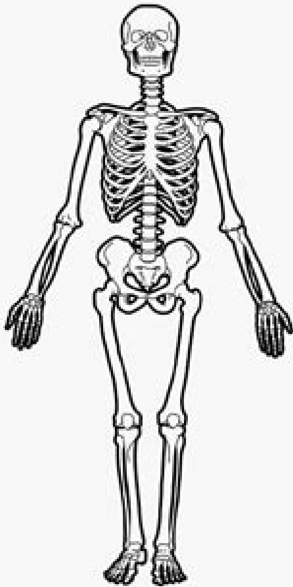
HTML
