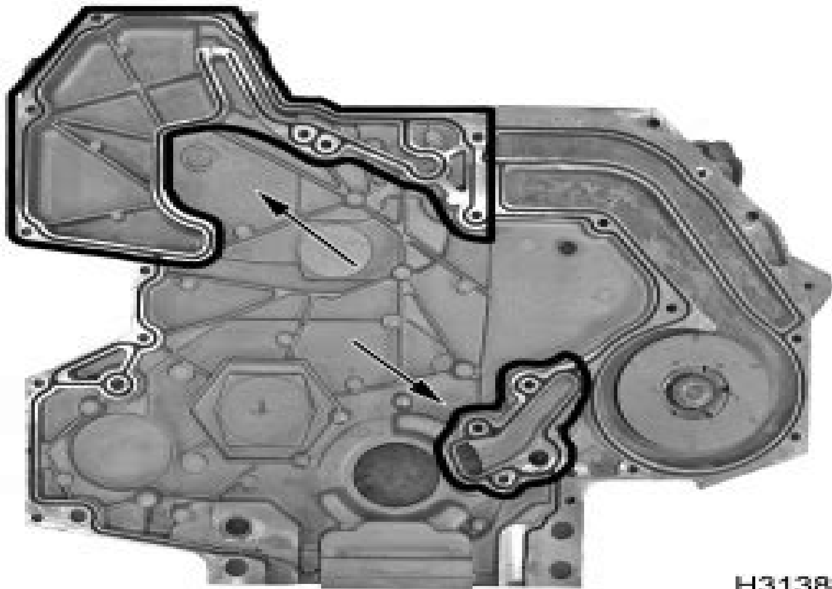
Figure 158 Front cover oil pressure leak locations
