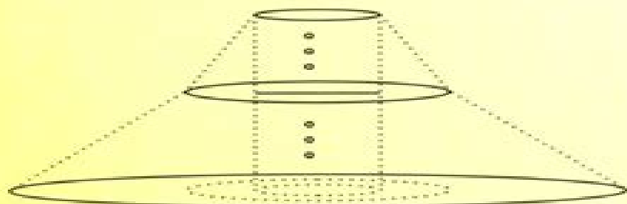
Abstraction hierarchy
