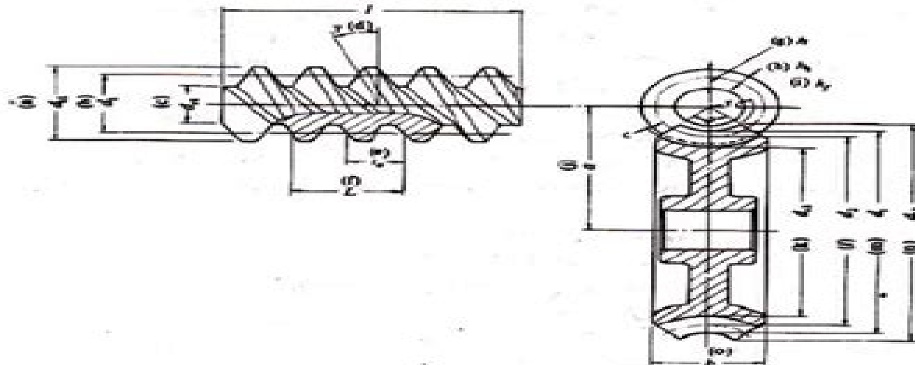
Gambar 1. Nama bagian-bagian roda gigi cacing.
